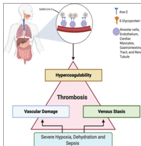
Figure 1: All three major contributors of Virchow's triad play a role in severe COVID-19 infection. Severe acute respiratory syndrome-associated coronavirus-2 utilizes S glycoprotein spikes to attach to angiotensin-converting enzyme-2 receptors found on multiple cell types in different organ systems. Vascular endothelium damage in this infection triggers rapid increase of pro-inflammatory cytokines resulting in cytokine storms in the patients. Hypercoagulability results due to the imbalance of procoagulant and anticoagulant pathways. The third-factor venous stasis is observed in critical cases as a result of immobility, shock, hypotension, and sedation
